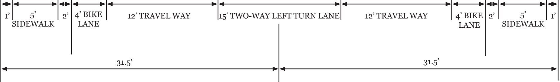
TYPICAL SECTION A
