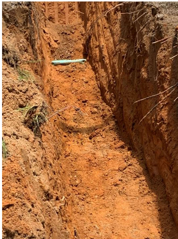
Photo 3: Service connection install
